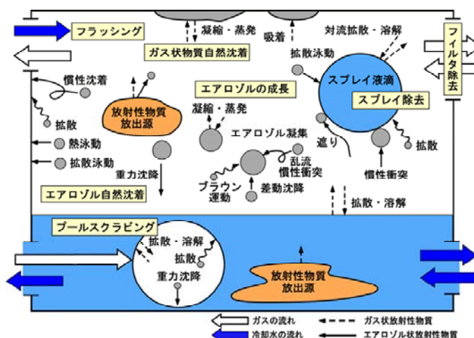
Figure 2. Radionuclide Behavior under Severe Accident Conditions
