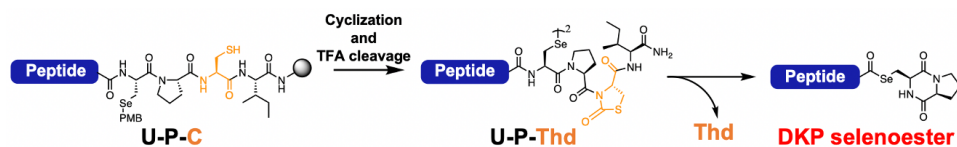
Fig 1. Scheme of peptide selenoester synthesis with diketopiperazine formation.
