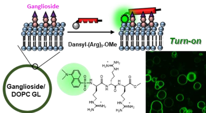
Figure 1. Illustration of fluorescence turn-on of Dansyl-(Arg) 3 -OMe on giant liposome of DOPC containing gangliosides.
