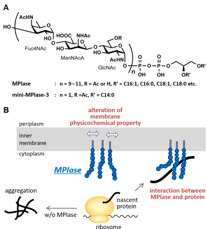
Fig 1. (A) Structure of MPIase and mini-MPIase-3. (B) Schematic illustration for the initial event of membrane protein integration in E. coli with MPIase. Glycans of MPIase capture nascent proteins and prevent them from aggregation.
