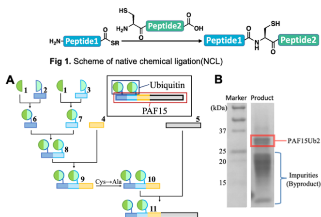
Fig 2. Synthesis of PAF15Ub2. (A) Ligation scheme of PAF15Ub2. (B) Result for SDS-PAGE analysis.
