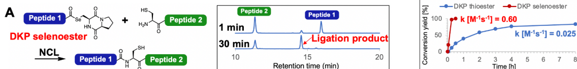
Fig 2. (A) Peptide ligation using peptide selenoester. (B) Kinetics studies of thioester and selenoester in NCL.
