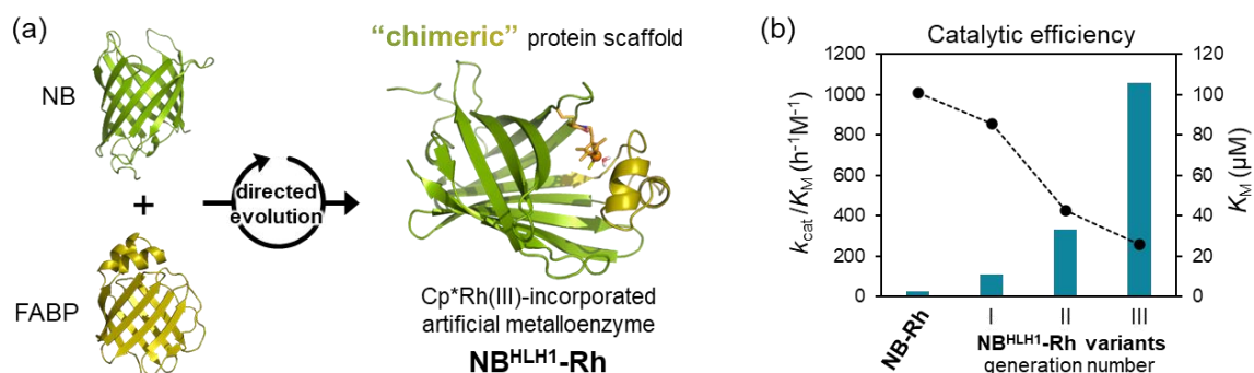
Figure 1. (a) Construction of a Cp*Rh(III)-linked artificial metalloenzyme with chimeric protein scaffold. (b) Michaelis-Menten parameters of evolved NB H1 -Rh variants for the cycloaddition reaction.
