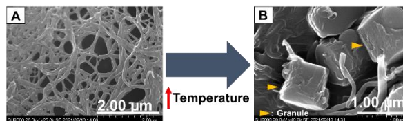
Fig. 2. Scanning electron microscopy micrographs of miRNA-based PICs: The fibrous structure (A) and granules (B).
