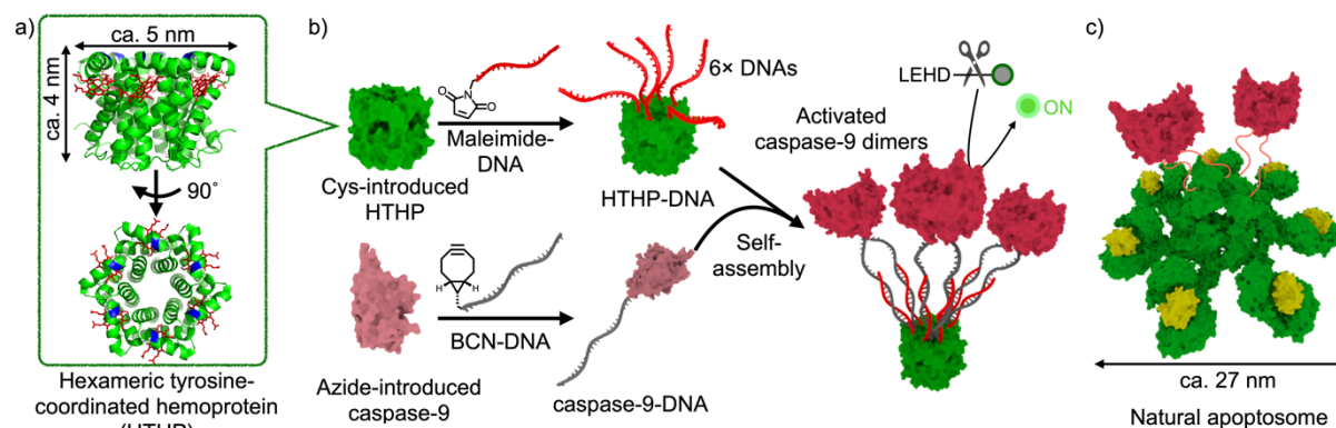
Figure 1. a) Crystal structure of HTHP (PBD ID: 2OYY), red molecules: heme b, blue parts: cysteine-introduced residue, V44. b) Schematic representation of preparation of ssDNA-introduced HTHP and Caspase-9 monomer (light red), and the assembled structure. Proximity-induced activity of caspase-9 dimers (deep red) is monitored using the Ac-LEHD-AFC substrate. c) Structure of the natural apoptosome that activates tethered caspase-9 via proximity-induced dimerization. Cytochrome c is indicated in yellow.
