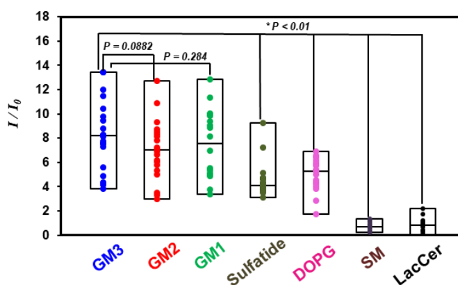
Figure 2. Box plot of fluorescence intensity distribution of 10 \mu\text{M} Dansyl-(Arg) 3 -OMe on DOPC giant liposomes ( N = 20 each) containing 40% gangliosides, sulfatide, DOPG, SM, or LacCer.
