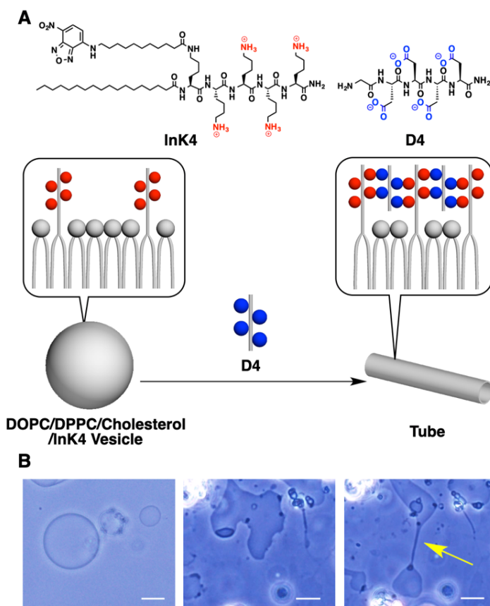
Figure. Schematic illustration (A) and micrographs (B) of the tube formation via the flattened object induced by self-assembly of the peptide receptor. Scale bars = 20 \mu\text{m} .
