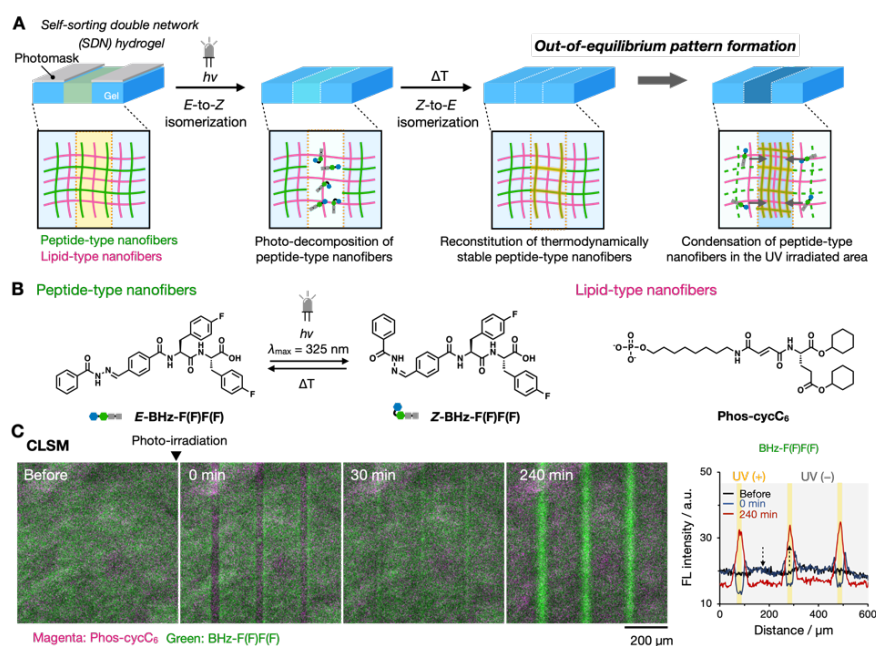
Fig. (A) Schematic illustration of this work (B) Chemical structures of the gelators (C) CLSM imaging of the out-of-equilibrium pattern formation
