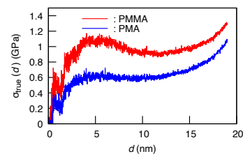
Fig.1 True stress-displacement curves of PMMA(red) and PMA(blue)
