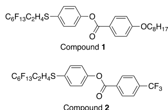
Figure 1. Chemical structures of compounds 1 and 2 .
