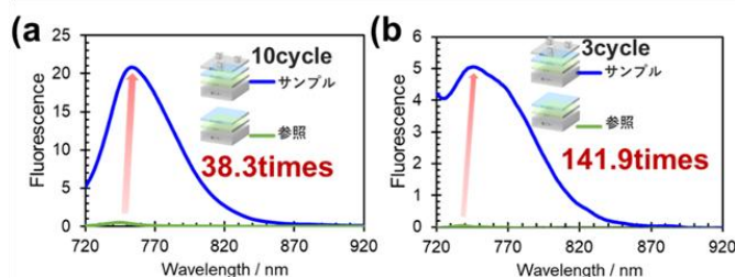
Fig. 1. Fluorescence spectra of MOFs/MIM prepared with spin-coating of (a) 10 and (b) 3 cycles.
