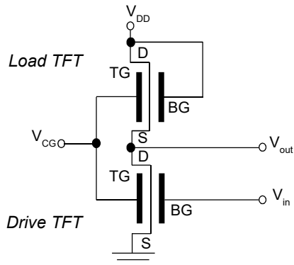
Fig. 4. E/E inverter circuit diagram in this research
