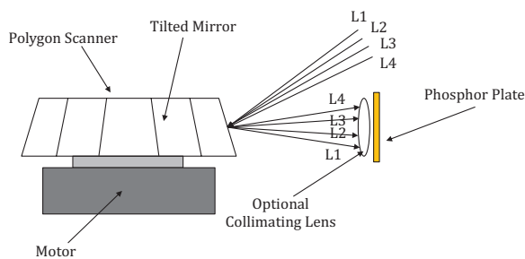
Fig. 3 Multiple Laser Headlight System
