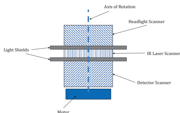
Fig. 1 Schematic Diagram of a 3-Level Integrated LiDAR/Headlight System
