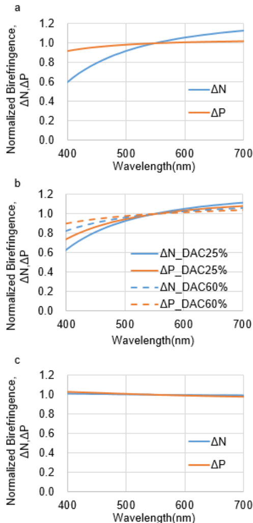
Fig. 3 Birefringence wavelength dispersion (a) New film (b) Acetyl Cellulose (c) COP.
