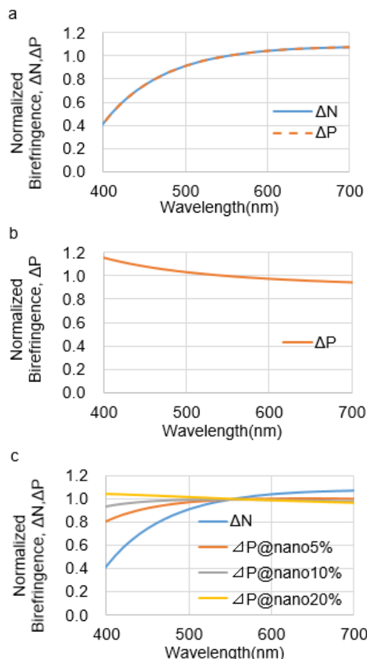
Fig. 2 Birefringence wavelength dispersion (a) polymer (b) nanoparticles (c) mixtures.
