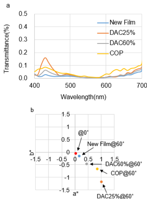
Fig. 5 Dark state light leakage of VA-LCD at the oblique angle (Azimuth 45°, Polar 60°) (a) Spectrum transmittance (b) Chromaticity ( a^*b^* ).
