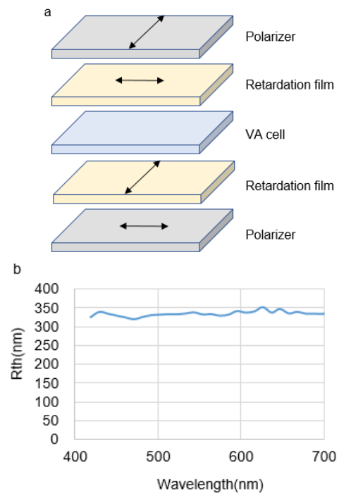
Fig. 4 Structure of VA-LCD (a) Optical configuration of VA-LCD (b) Rth of the commercial VA-LCD
