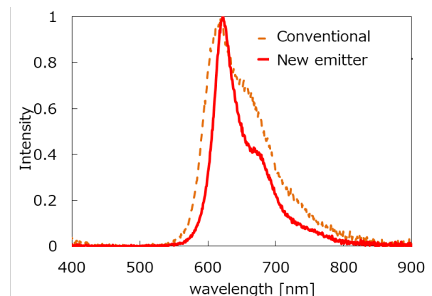
Fig. 6. Photoluminescence spectra
