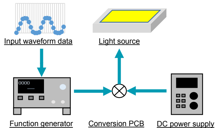
Fig. 2 Light source system configuration
