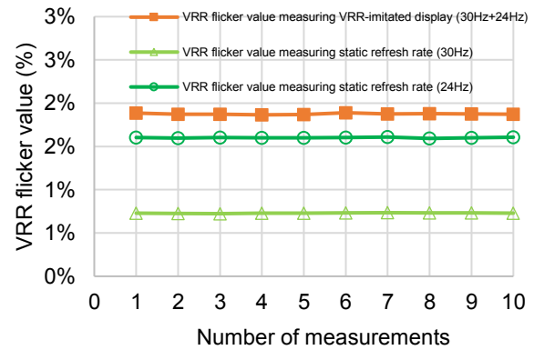
(b) Measured VRR flicker value
