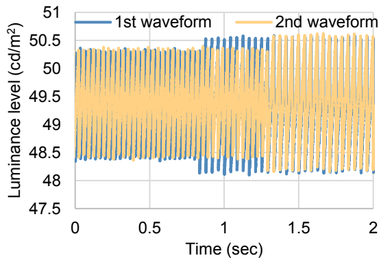
Fig. 4 Waveform emission samples that phase shift
