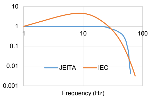
Fig. 1 TCSF from JEITA flicker method and IEC 62341-6-3:2017 corrigendum 1
