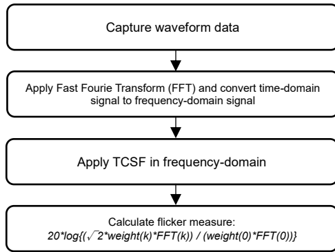
(a) JEITA flicker method
