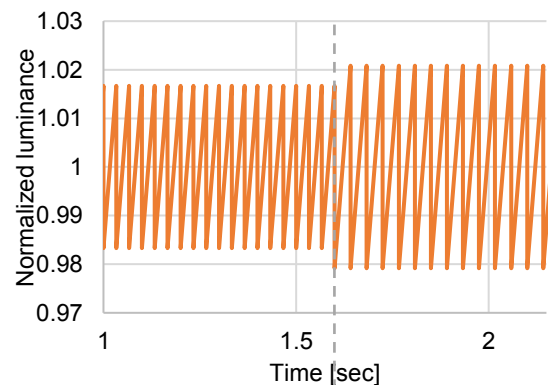
(a) Waveform emission overview
