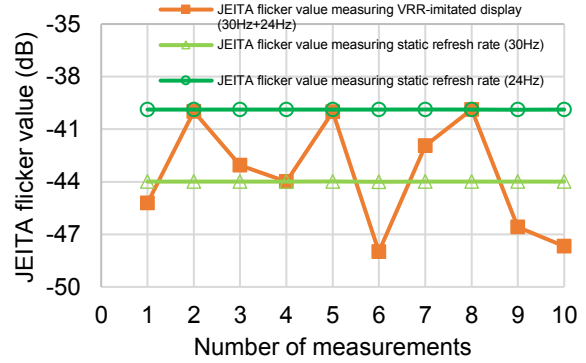
(a) Continuously measured JEITA flicker value
