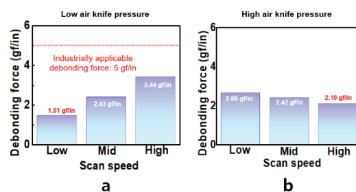
Fig. 1 Minimization of mechanical debonding force by the optimal coating of the 2D material-based debonding layer under a low air knife pressure, and b high air
