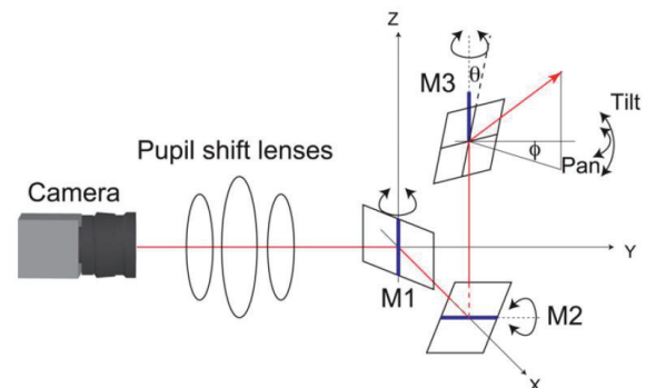
Fig.1 Structure of Saccade Mirror 3[4].
