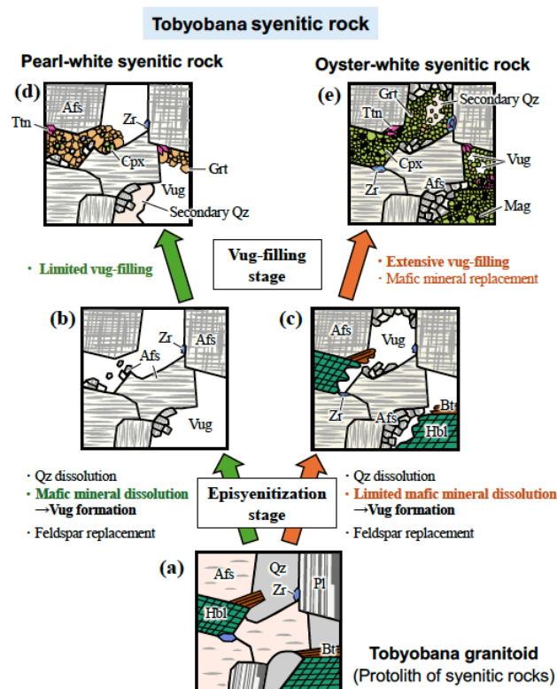
Figure Schematic illustration showing the model for the formation of two contrasting syenitic rocks in the Tobyobana area. See text for explanation. (a) Tobyobana granitoid (protolith of syenitic rocks). (b) Quartz and mafic mineral dissolved Tobyobana granitoid (i.e., pearl-white syenitic rock before vug-filling). (c) Quartz dissolved Tobyobana granitoid (i.e., oyster-white syenitic rock before vug-filling). (d) Pearl-white syenitic rock. (e) Oyster-white syenitic rock. Qz: quartz, Afs: alkali feldspar, Pl: plagioclase, Bt: biotite, Hbl: hornblende, Cpx: clinopyroxene, Grt: Garnet, Ttn: Titanite, Zr: Zircon, Mag: Magnetite.
