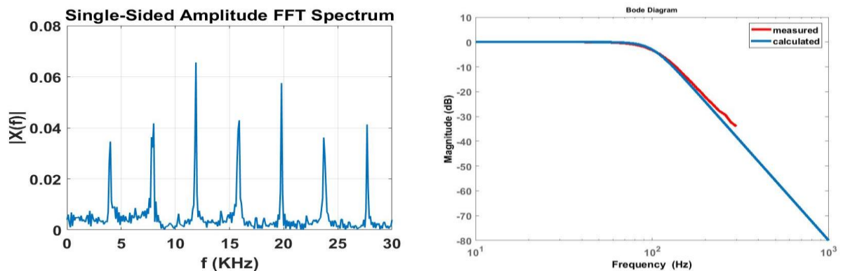
FIGURE 7. (a) FFT spectrum of the unfiltered torque signal. (b) Frequency response of a fourth order Butterworth filter
