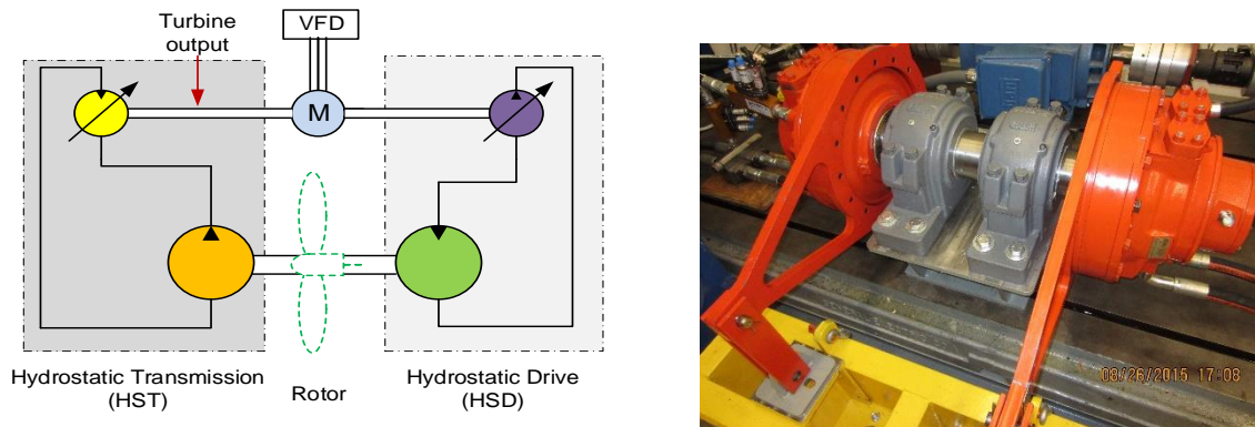
FIGURE 4. (a) Schematic of Power Regenerative Test Platform (b) Rotor Assembly
