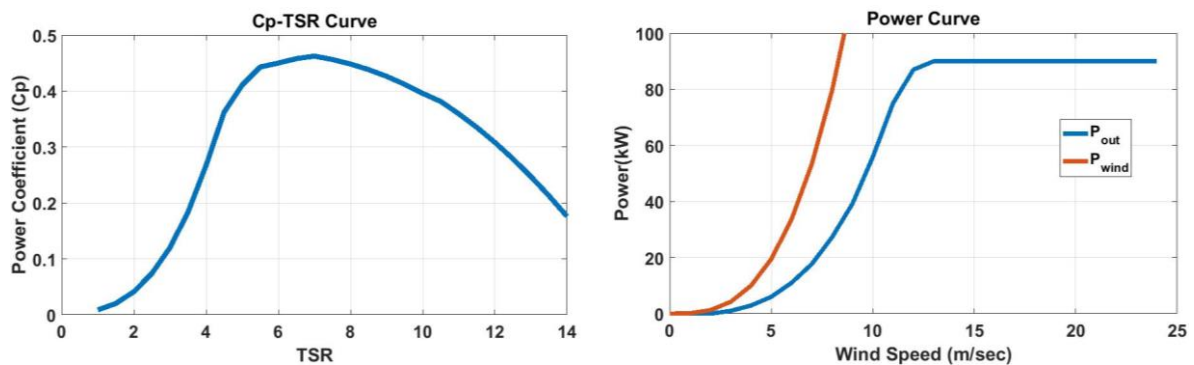
FIGURE 1. (a) Power coefficient curve of a three bladed variable speed turbine. (b) Power curve of a 90 kW wind turbine.
