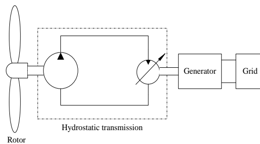
FIGURE 3. Schematic of HST wind turbine
