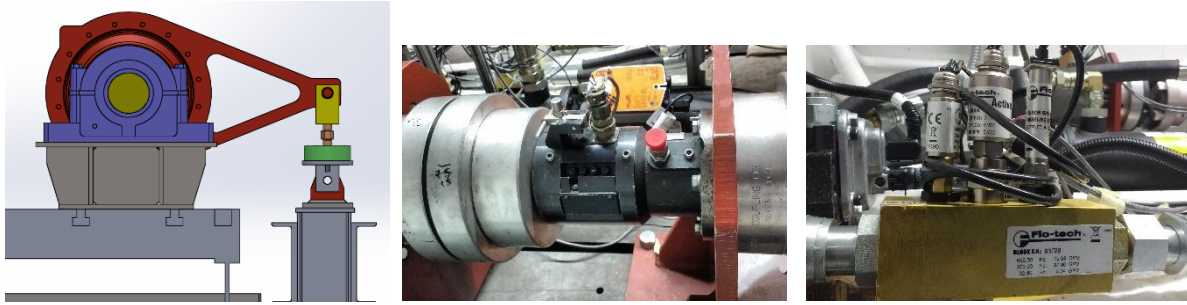
FIGURE 6. (a) Load Cell Assembly. (c) Rotary torque sensor (b) Flow sensor Module
