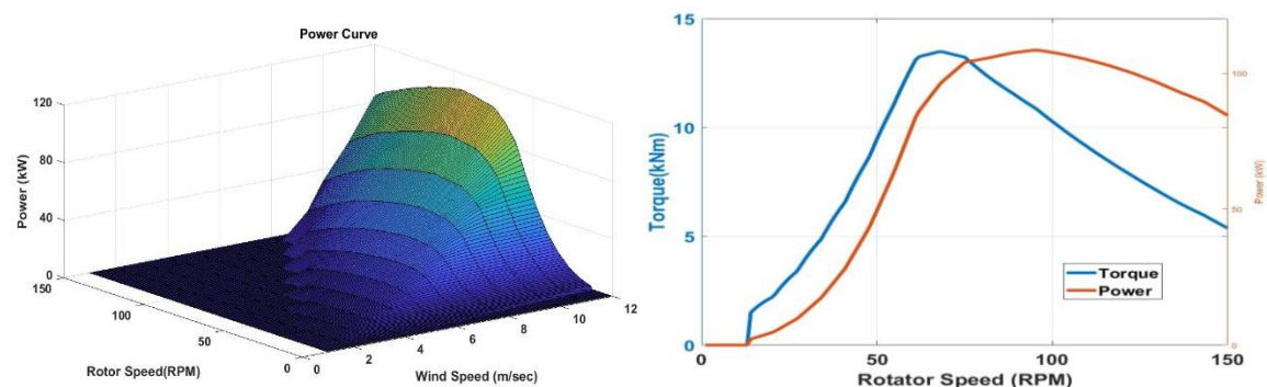
FIGURE 2. (a) Rotor Power curve (b) Rotor torque and power at rated speed (12 m/sec)
