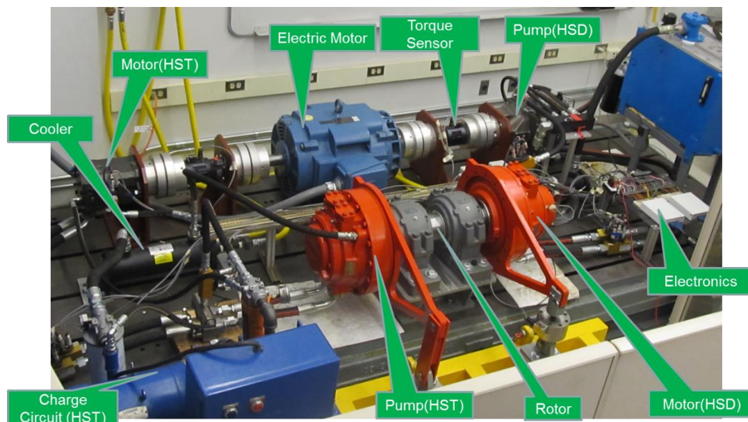
FIGURE 5. Power Regenerative Test Platform
