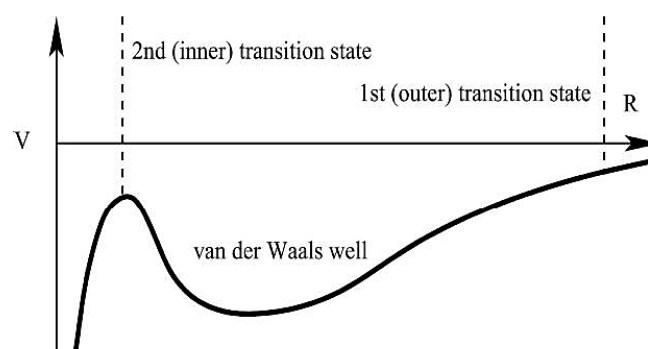
Figure 1. Schematic one-dimensional picture of the potential energy as a function of the reaction coordinate for a neutral-neutral reaction leading to bimolecular products. In its approach, the 2TS model incorporates both the 1 st (outer) transition state for barrierless association reaction and the 2 nd (inner) transition state for reaction path with a barrier. Source: Georgievskii and Klippenstein, 2007.
