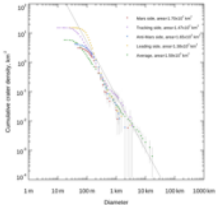
Figure 2. The cumulative crater size-frequency distribution. Each color represents the following areas. Red: Mars side, purple: trailing side, blue: anti-Mars side, yellow: leading side, green: average (PH9224GT).
