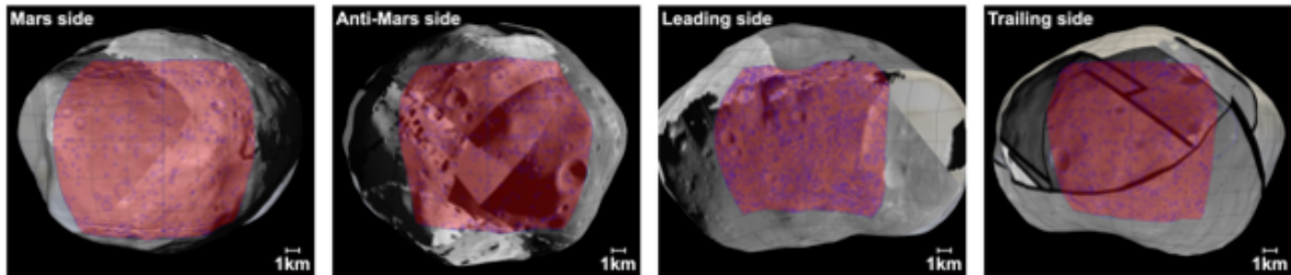
Figure 1. The 4 categories of Phobos (between 30° N and 30° S): Mars side (330°–360° W, 0°–30° W), anti-Mars side (150°–180° W, 180°–210° W), leading side (60°–90° W, 90°–120° W), and trailing side (240°–270° W, 270°–300° W). The circles represent the results of crater counting.
