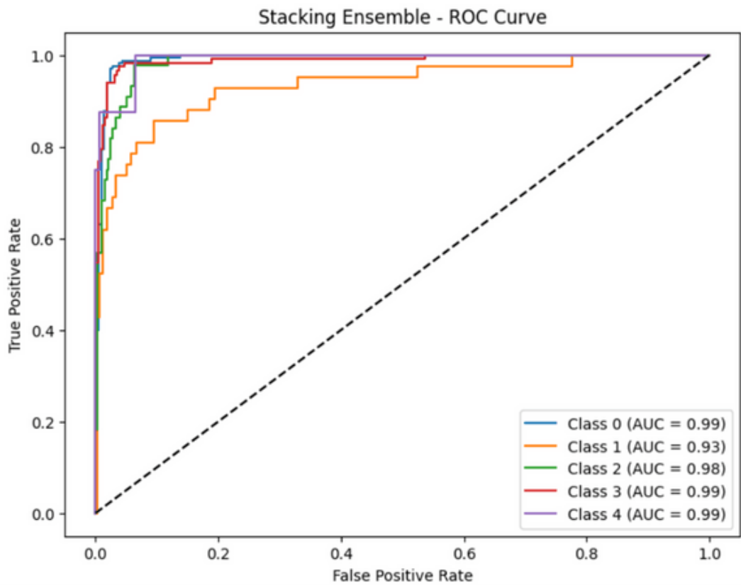
Figure 2: Receiver Operating Characteristic (ROC) curves for the stacking ensemble model visualizes the diagnostic ability of the multi-class classifier by mapping the true positive rate against the false positive rates at various threshold settings.
