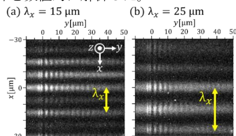
Fig 1. Optical micrographs for striped ST-SPPs with (a) \lambda_x \approx 15 \mu\text{m} , and (b) 25 \mu\text{m} .
