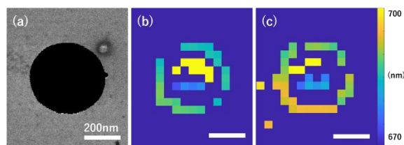
Fig.2 (a) Si particles with the diameter of 400 nm. (b) WGM spectrum peak mapping without laser irradiation. (c) WGM spectrum peak mapping under 40 μW laser irradiation.
