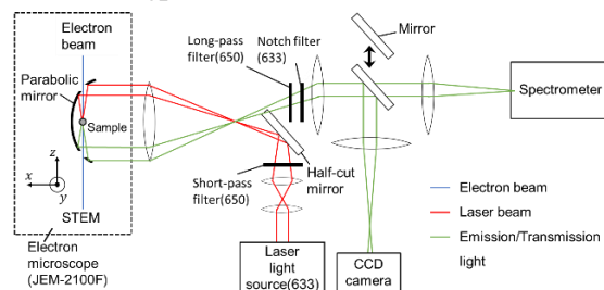
Fig. 1 Experimental setup for simultaneous irradiation of electron beams and laser beams.
