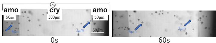
Fig.3: Polystyrene particles 3 \mu\text{m} and 5 \mu\text{m} in diameter separated by the crystalline phase area (white area) on GST substrate under ICEO influence
