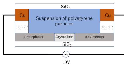
Fig.1: Schematic diagram of the experimental setup
