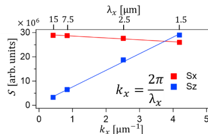
Fig 3. Correlation between \lambda_x and the maximum values of S_x and S_z .
