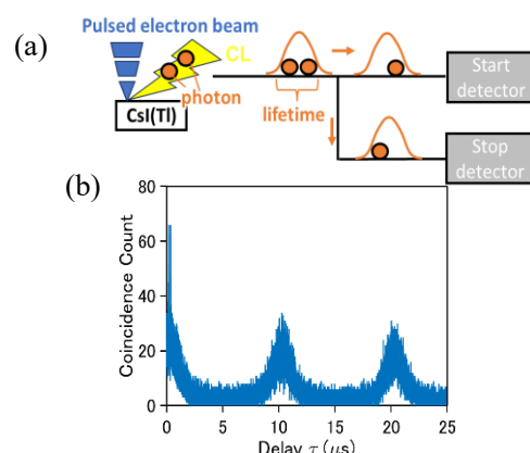
Fig.1(a) Measurement system. (b) Result of HBT measurement using CsI:Tl by pulsed electron beam.
