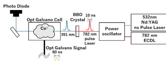
Fig. 1. Experimental setup.
