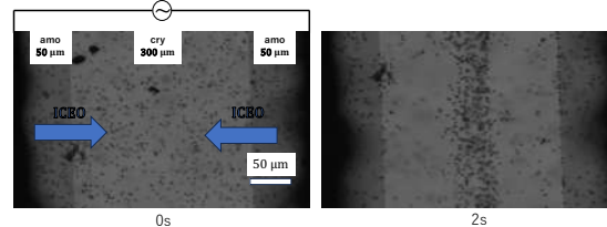
Fig.2: Polystyrene particles of 3 \mu\text{m} diameter gathered in the crystalline phase area (white area) on the GST substrate under the influence of ICEO.
