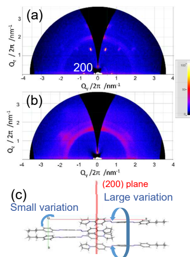
Figure 2. The GI-WAXS patterns of the incident light (a) perpendicular to and (b) parallel to rubbing direction. (c) The molecular packing in the films.
