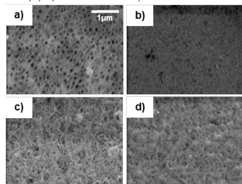
Fig.2 SEM images of 1:2 blend films (PEDOT:PSS / Polymer = 1:2 blend): (a) NIPAM / SSNa = 100:0, (b) 76:24 (c) 54:46 and (d) 29:71.
