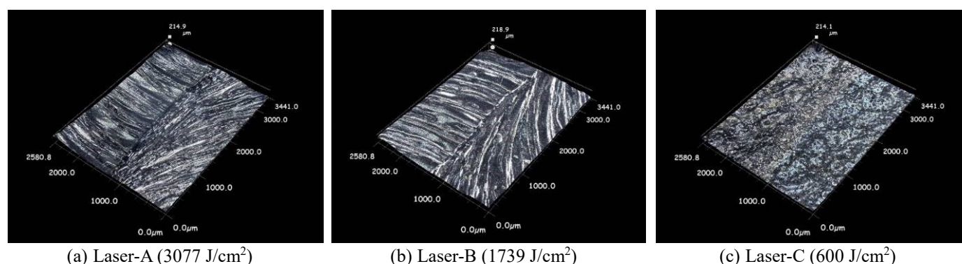
Fig.1 Surface of laser-treated carbon steel plate
