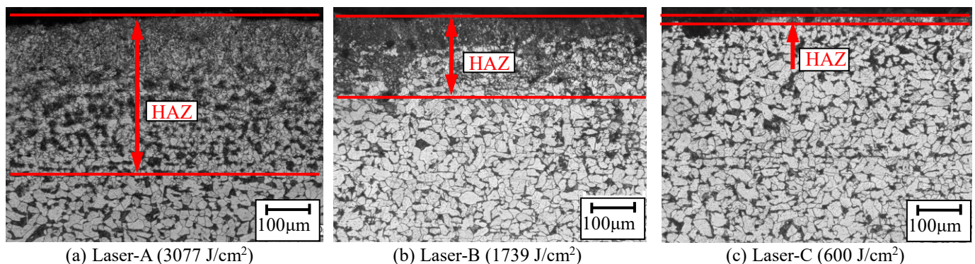
Fig.3 Microstructure of laser-treated carbon steel
