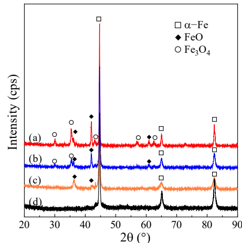
Fig.2 XRD diffraction patterns of specimens: (a) Laser-A, (b) Laser-B, (c) Laser-C, (d) Unirradiated
