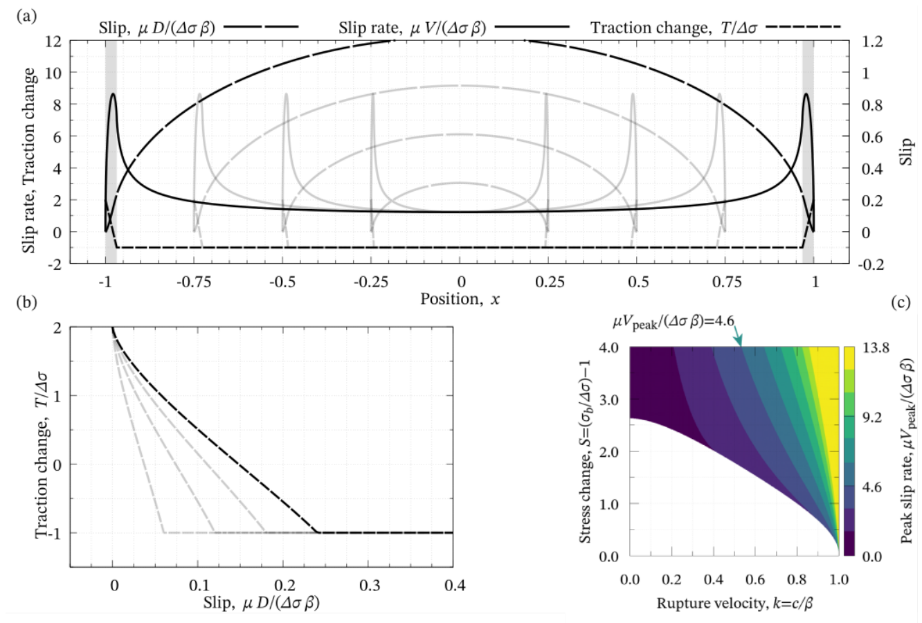
(a) Slip, slip rate, and traction on the fault for S=2 and k=0.9 . Curves for ct = 0.25, 0.5, 0.75 (gray), and 1.0 (black) are plotted. (b) Slip-stress curve for S=2 and k=0.9 . Curves for x = 0.25, 0.5, 0.75 (gray) and 1.0 (black) are plotted. (c) Normalized peak slip rate as a function of S and k . The blank region indicates absence of solution that satisfies V(\pm 1)=0 .
