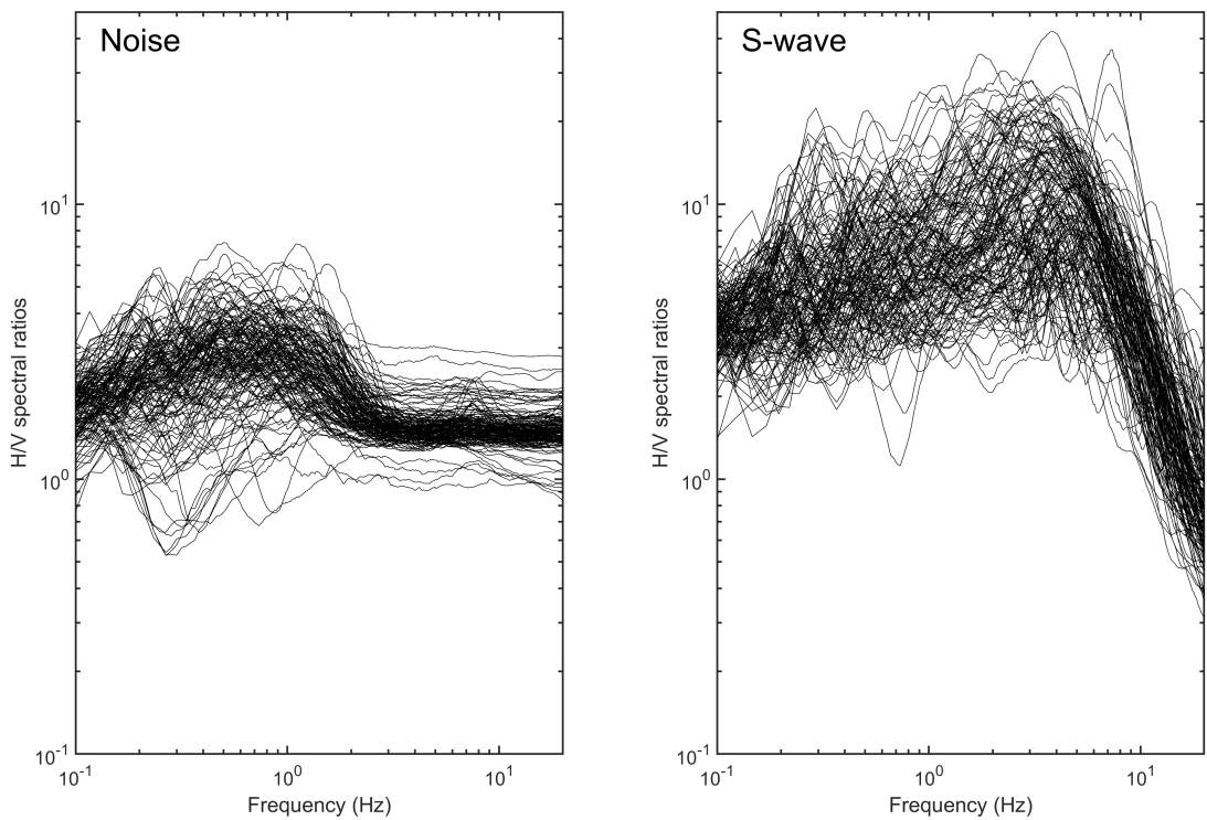
Median values of H/V spectral ratios at the S-net sites
