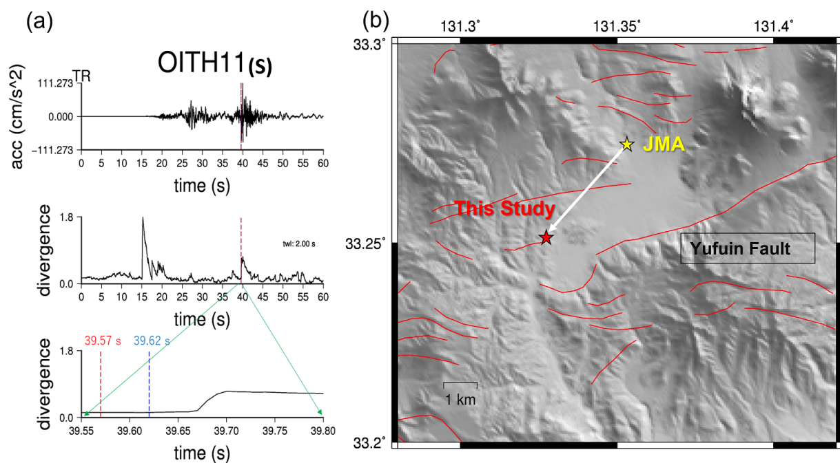
Figure 1. (a) An example of S-wave picking in OITH11. Red and blue dashed lines indicate arrival times of S-wave picked in this study (39.57 s) and reported by JMA (39.62 s), respectively. (b) Location of the triggered earthquake in this study. Red and yellow stars denote epicenters determined in this study and reported by JMA, respectively. Each of Red lines indicates the active fault in this region.
