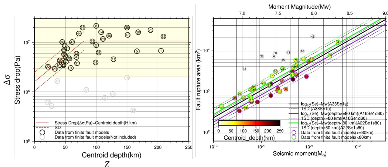
Fig1. (a) Black circles show the relationship between stress drop and Centroid depth. The red solid line and broken line at a depth shallower than 80km are the regression line and standard error derived from data, respectively. A Red solid line at a depth deeper than 80km indicates the averaged stress drop. (b) Solid lines show the scaling relation for moment magnitude and fault rupture area for intraslab earthquake. The fill color of circles shows the centroid depth for earthquakes. Gray circles show the magnitude and fault rupture area of those earthquakes whose stress drop are smaller than 2MPa. These earthquakes are not used in the regressions. Green and purple circles are the earthquakes whose centroid depth is shallower and deeper than 80km, respectively. Green and purple lines are the regression lines for the data with the same color. The black line is the regression line for all data except for the gray circle.
