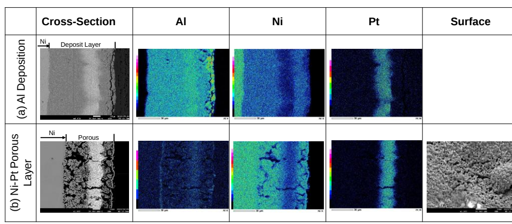
Fig. 1 Cross-sectional structure of a sample on which Al was deposited after Ni and Pt plating (a), and a porous sample (b).
