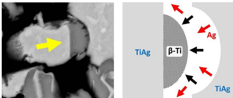
Fig. 1. Schematic of the liquid film migration mechanism.
